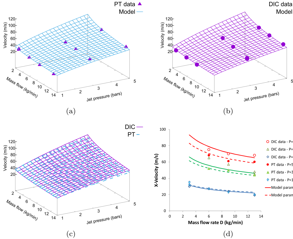
Fig. 16 Stable velocity V_X^{stable} ( m/s ) as a function of the jet pressure P and the mass flow rate D , a PT: data vs calibrated model, b DIC: data vs calibrated model, c Comparison of the calibrated models using PT and DIC data, d Cut at a given jet pressure. DIC and PT data vs calibrated model
