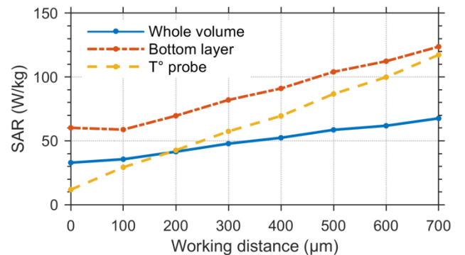
Fig. 4. Variation of SAR values (whole volume, bottom layer at the cells level, Luxtron temperature probe) versus the microscope objective position (0 \mu m and 100 \mu m correspond to the working distance of the 63x and 20x objectives, respectively). SAR values are normalized per 1 W incident power.
