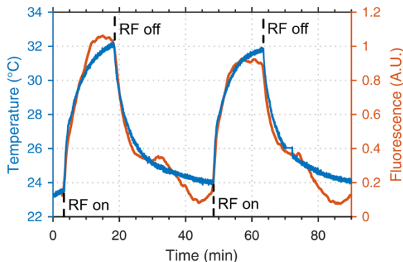
Fig. 5. Experimental results of temperature versus Rhodamine B fluorescence variation obtained with the 20x objective. The biological samples (3ml of 50 \mu M Rhod B in HBSS) are exposed to 1.8 GHz, 20 W incident power for twice a duration of 15 minutes.
