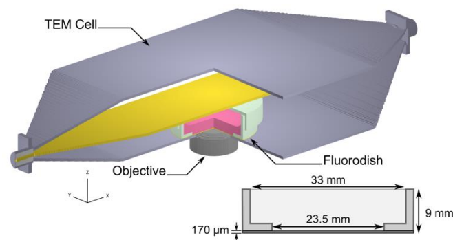
Fig. 2. TEM cell with a FluoroDish that contains the biological sample (numerical model extracted from FDTD software, FluoroDish dimensions).
