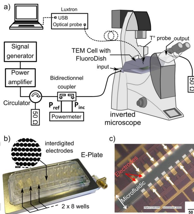
Fig. 1. Biological sample EMF exposure, temperature measurements setup and real-time microscopic measurements of Rhodamine B fluorescence. a) TEM cell with FluoroDish. b) Microsystem with thin interdigitated array electrodes c) Microfluidic chip.
