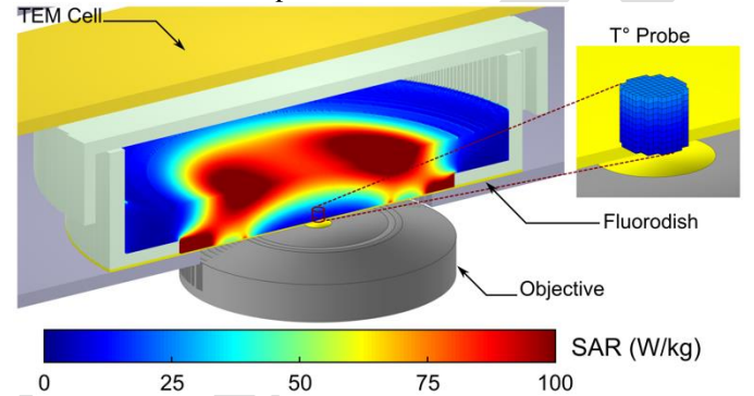
Fig. 3. SAR spatial distribution within the biological sample inside the FluoroDish placed in the TEM cell. In the inset, the SAR Probe 1-mm cylinder for comparisons with Luxtron probe measured SAR. SAR values are normalized per 1 W incident power.
