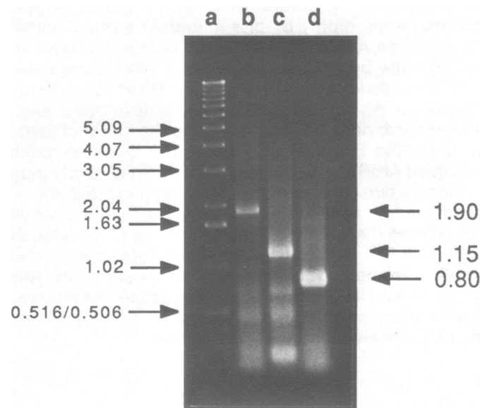
Figure 2: Agarose gel electrophoresis of PCR extension products. PCR amplifications were performed using the oligonucleotide primers described in Fig. 1. One tenth of the final polymerization mixtures was fractionated on a 1% agarose gel. Numbers refer to sizes in kbp. Lane a, DNA ladder. Lane b, amplification of the 1.9 kbp was achieved using primers AP1 and AP4 which create Hind III sites at both ends (to clone into pUC18 vector). Lanes c and d, the amplification of the gene was also performed using primers AP1–4 to produce two DNA fragments of 0.8 and 1.15 kbp, overlapping each other on a 50 bp central region which contains a unique Sph I restriction site.
