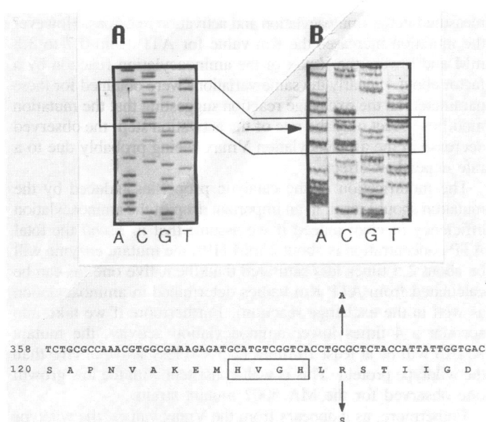
Figure 3: Sequences showing the location of the mutation in ArgRS from strain MA5002. The entire 1.9 kbp Hind III fragment was sequenced using primers 1–6. The autoradiographs shows sequences of argS from strain MA5002 (B) and wildtype (A) in the region of the mutation. The position of the mutation is indicated by an arrow. Below, the mutation is indicated on the mRNA identical DNA strand and results in a Arg (C) to Ser (A) change at codon 134.
