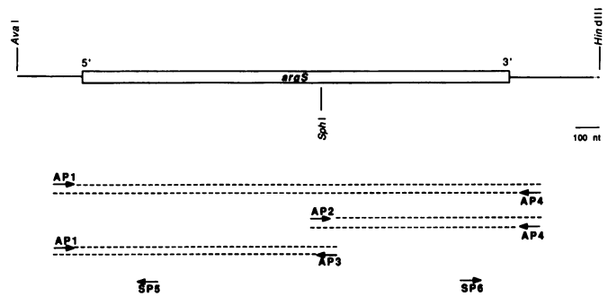
Figure 1: Amplification and sequencing strategy of the argS region.
