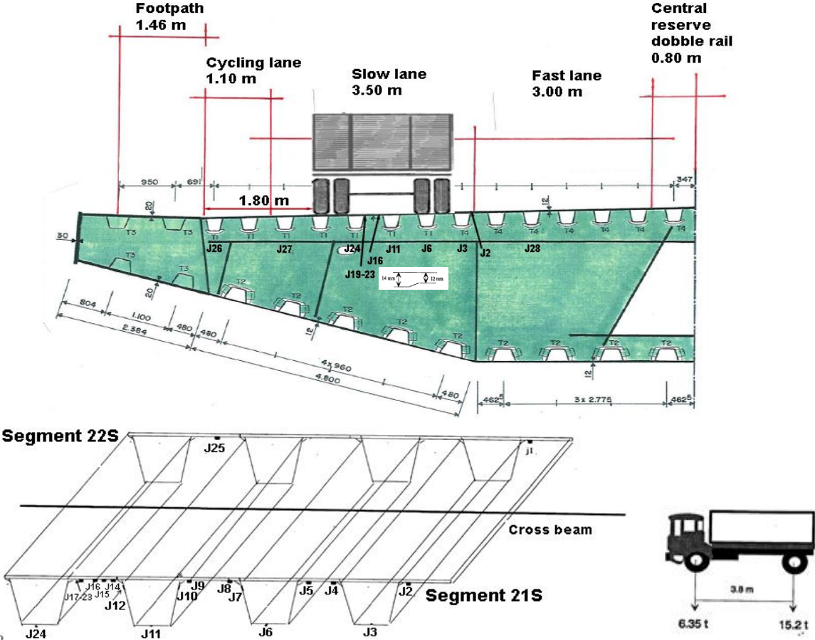
Figure 2 – Bridge of Normandy, transverse cross section, stain gauges and test truck (1995)
