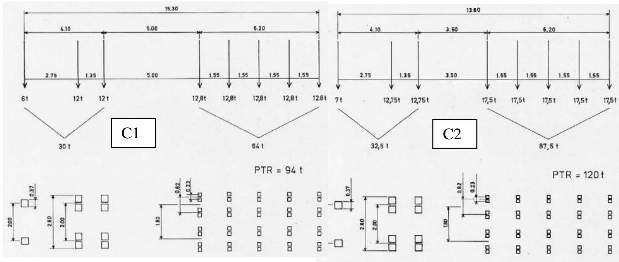
Figure 6 – Abnormal loads: (G1) (G2) cranes 98 t - 108 t, (C1) (C2) vehicles 94 t - 120 t
