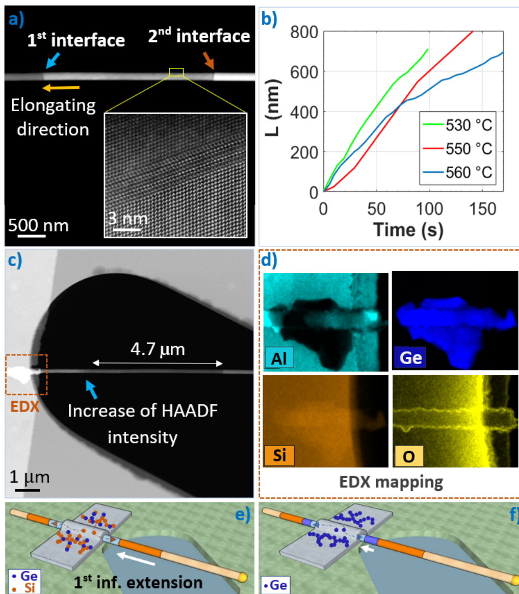
Figure 2 | Real time observation of the thermal exchange between Al pads and a \text{Si}_{0.67}\text{Ge}_{0.33} NW during the cooling process. a) HAADF-STEM image of a NW propagated at 560 ^{\circ}\text{C} during the cooling process, showing the movement of the first interface in the reverse direction toward the Al contact pad. The inset figure shows the zoom on the rectangular yellow box, demonstrating the formation of crystal defects in the newly formed NW region. b) The plot of the first interface diffusion length ( L ) in reverse direction as a function of time at three different cooling temperatures, showing a linear diffusion behavior. c) HAADF STEM image after 4.7 \mu\text{m} of backward propagation where an increase of HAADF intensity is observed in the created region, as well as the formation of a large crystal when the first interface reached the Al contact pad. d) EDX mapping on the created large crystal (indicated by the orange dashed box) at the Al contact pad showing the main contribution of Ge in the crystal composition. The in-situ video of the first interface during the cooling process (at 560 and 500 ^{\circ}\text{C} ) are presented in the supporting
