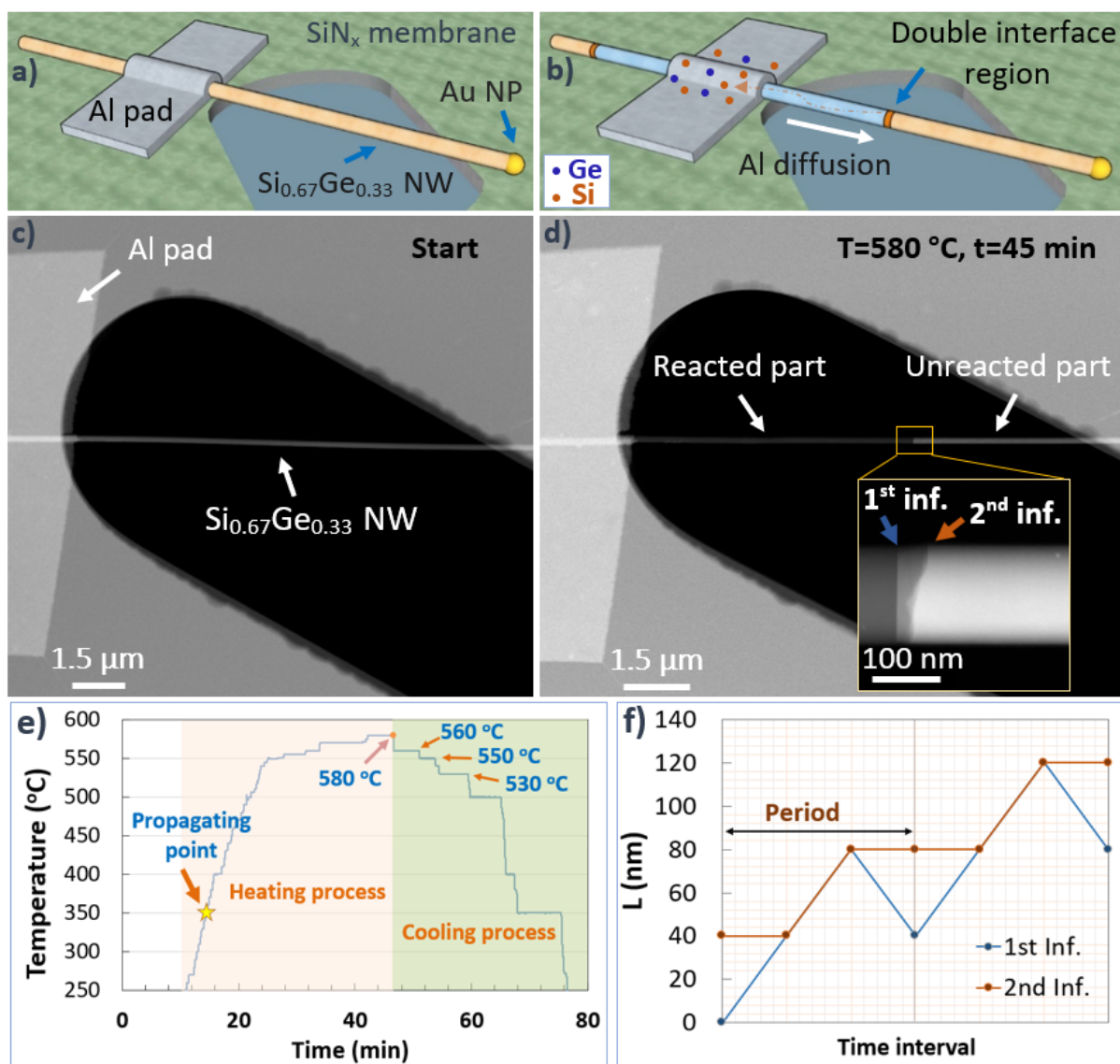
Figure 1 | Real time observation of the thermal exchange between Al pads and a Si 0.67 Ge 0.33 NW during the heating process. a-b) Schematic illustrations of the contacted NW before and after annealing for 45 min. Si and Ge atoms are displayed in orange and blue colors, respectively. The white arrow in Fig. 1b shows the propagating direction of the reaction interface while the orange arrow shows the diffusion of Si and Ge atoms in the opposite direction. c-d) HAADF STEM images of the Al contacted Si 0.67 Ge 0.33 NW crossing over the 6 μm x 23 μm hole of a SiN x membrane before and after the in-situ heating experiment. The diameter of the contacted NW is about 150 nm with a length of 20 μm. The insert in Fig. 1b shows the presence of a double interface region, sandwiched between the Al reaction part and unreacted Si 0.67 Ge 0.33 part. e) The plot figure shows the heating temperature as a function of time during the heating and cooling process. f) The schematic illustration for the relative positions of the first and second interface during the propagation time. A real time propagation of Al/ Si 0.67 Ge 0.33 interface is presented in the Supporting Information SI M1.
