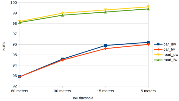
Fig. 5: IoU of road and car classes with different depth thresholds. All pixels with a depth value superior to the threshold are ignored in the IoU computation.
