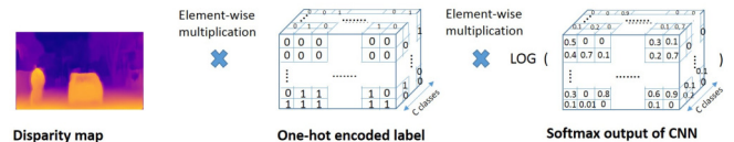
Fig. 1: Disparity weighting: Each pixel in the cross-entropy loss function is weighted by its value in the disparity map.
