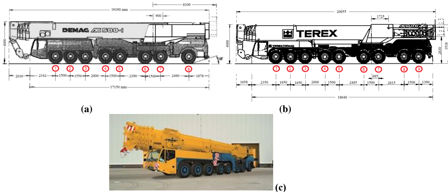
FIGURE 5 Abnormal loads: Cranes, (a) 96 tons, (b) and (c) 108 tons
