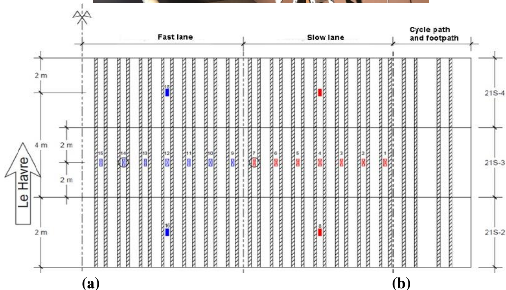
18 19 20 FIGURE 3 (a) Extensometers of the SiWIM fixed under each longitudinal stiffener, (b) 21 mapping of the instrumentation.
