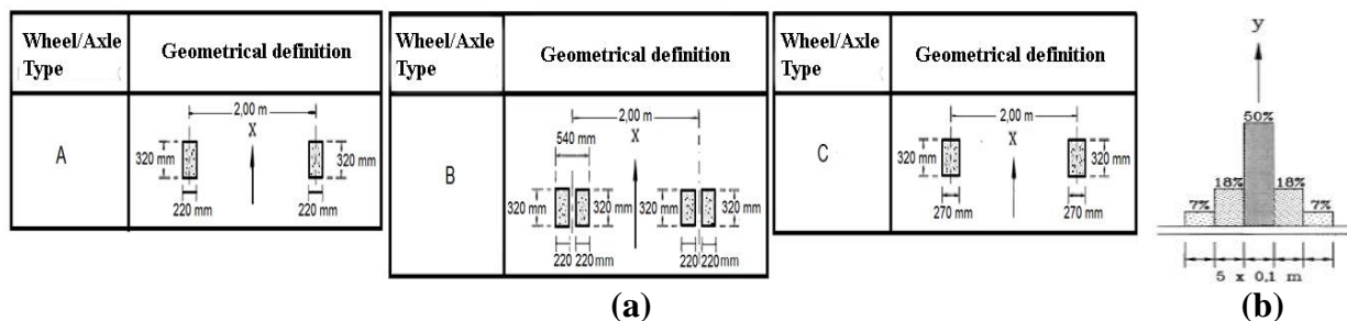
FIGURE 9 (a) Types of wheel/axle for load application, (b) statistical transversal distribution of the wheels in the traffic flow, both according to the EN1991-2.
