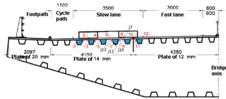
30 FIGURE 8 (a) Sections (locations) of the calculated influence lines (1 to 12 in red), (b) Transverse 31 locations of the (middle of) axle in the slow lane for the calculation of the influence lines.
