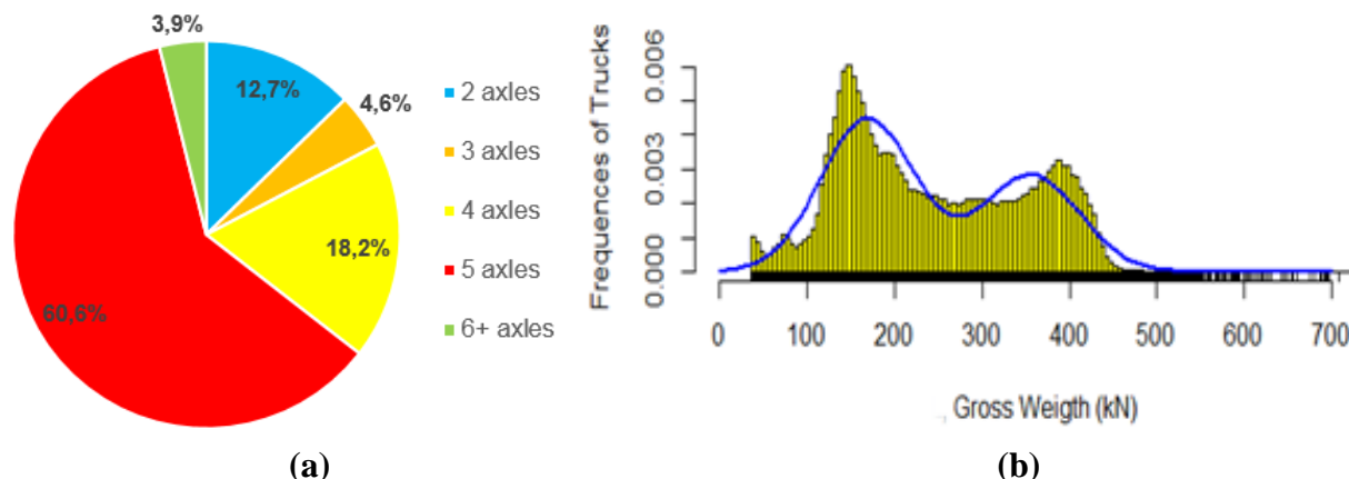
FIGURE 4 Traffic on Normandy bridge (July 2017- January 2018): (a) Truck distribution by category, (b) Gross vehicle weight PDF.
