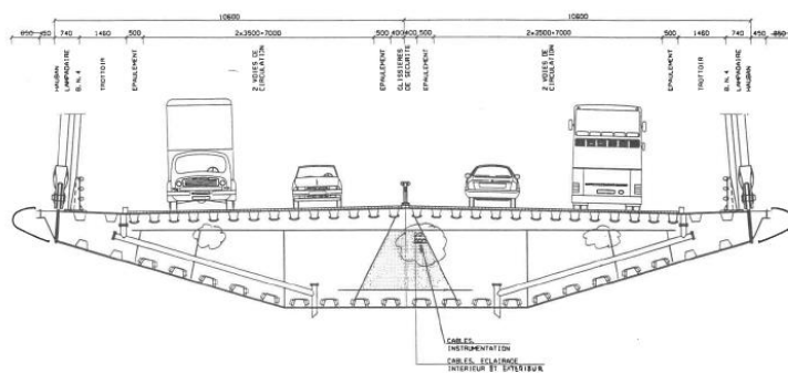
26 27 (a) (b) 28 FIGURE 2 Bridge of Normandy: (a) cross section of the steel orthotropic deck, (b) inside of the box.
