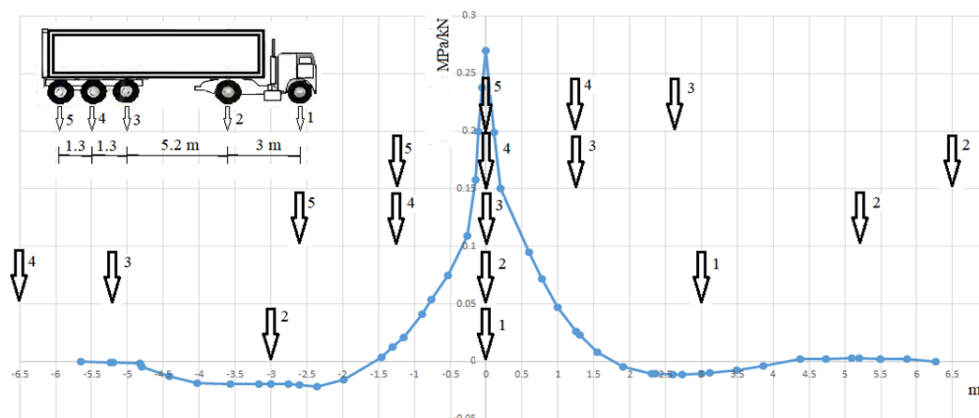
FIGURE 11 Assessment of the rain-flow histogram for a simple loading case: 5-axle articulated truck (axle loads 7, 12, 7-7-7 tons).
