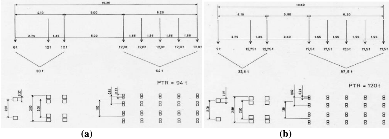
FIGURE 6 Abnormal loads and wheel layout: (a) C1 94 tons, (b) C2 120 tons
