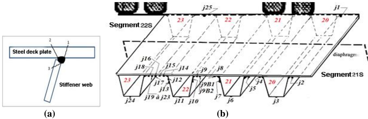
12 FIGURE 7 Normandy bridge deck: (a) weld between the deck plate and a longitudinal stiffener web, 13 and expected cracks under fatigue (named 1, 2 and 3), (b) Instrumentation of the deck with strain 14 gauges (1995).
