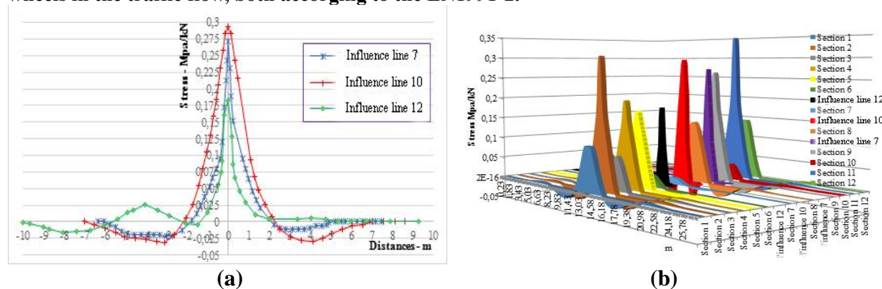
FIGURE 10 Influence lines of the critical details: (a) measured in 1995, (b) calculated by FEM in 2016.
