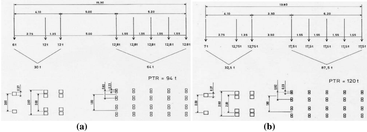
13 14 (a) (b) 15 FIGURE 6 Abnormal loads and wheel layout: (a) C1 94 tons, (b) C2 120 tons
