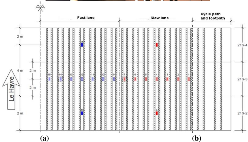
18 FIGURE 3 (a) Extensometers of the SiWIM fixed under each longitudinal stiffener, (b) 19 mapping of the instrumentation. 20 21
