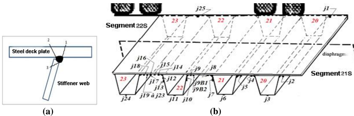
10 11 12 FIGURE 7 Normandy bridge deck: (a) weld between the deck plate and a longitudinal stiffener web, 13 and expected cracks under fatigue (named 1, 2 and 3), (b) Intrumentation of the deck with strain 14 gauges (1995).
