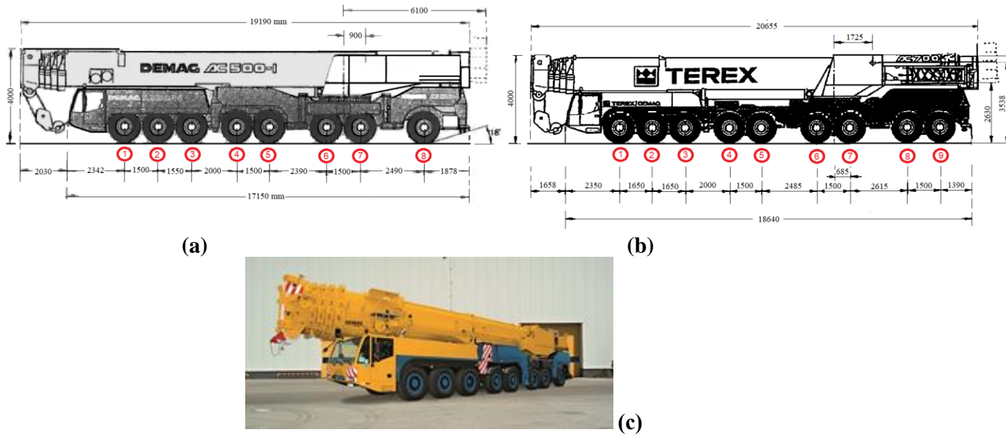
9 10 (a) (b) 11 (c) 12 FIGURE 5 Abnormal loads: Cranes, (a) 96 tons, (b) and (c) 108 tons
