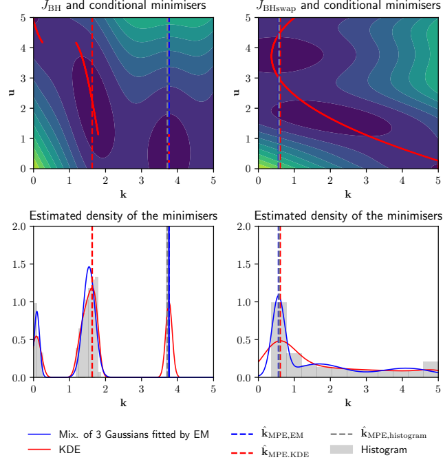
Figure 2: Top Left: J_{BH} along with conditional minimisers in red. Bottom left: Estimated densities using KDE and EM algorithm and the histogram. The dashed lines indicate the MPE found using those methods. Right: Same quantities with J_{BHswap} .
