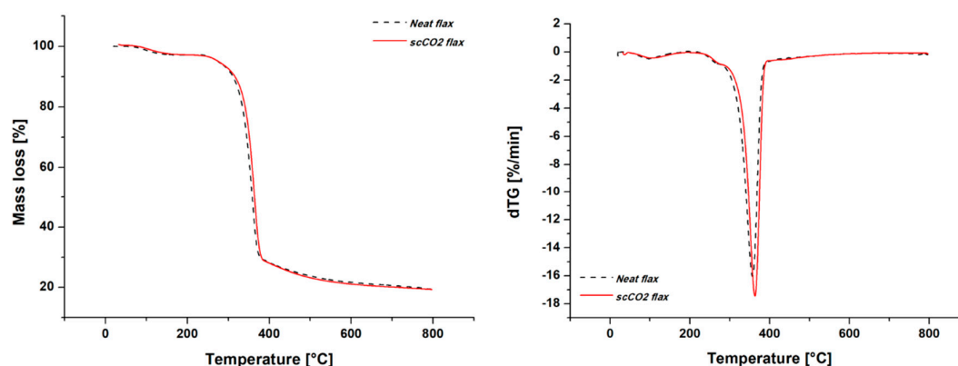
Figure 4. TGA thermograms and derivative thermogravimetry (dTG) curves of flax yarns before and after \text{scCO}_2 treatment.
