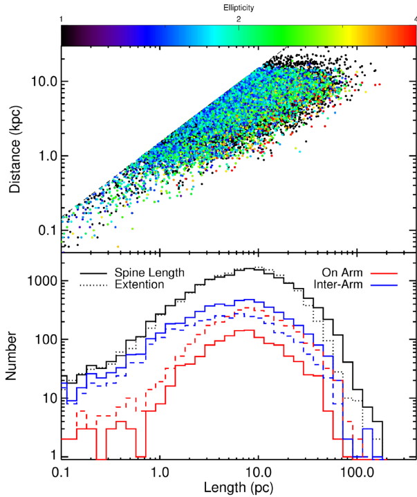
Figure 24. Top panel: Relation between the filament’s physical length and its assigned distance. The dashed line outlines the size corresponding to the cut-off criteria introduced in Section 4.1. Structures are shown with a colour code associated with their relative ellipticity e . Lower panel: distributions of the physical sizes of the Hi-GAL filaments. The physical sizes are determined from two estimators (see Section 4.3): the length of the main axis, or angular length, l^a (solid line) and the angular extension of the extended mask l^e (dotted line). The red and blue lines show the l^a distributions for features associated with Galactic spiral arms and inter-arm regions, respectively, for arm sizes of W = 600 pc (solid lines) and W = 1 kpc (dashed lines).
