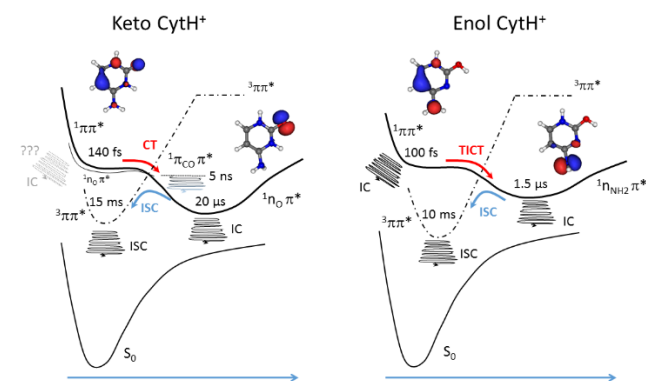
Figure 7. Schematic PES, excited state lifetimes and proposed deactivation mechanisms to the ground state for keto and enol CytH + .
