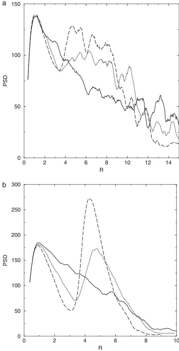
Fig. 4 The pore size distribution (PSD) versus pore radius R . a Effects of density of impurities on PSD at \phi_m = 0.173 , R_t = 4 ; the solid, dotted, and dashed lines correspond to \phi_i = 0 , \phi_i = 0.15 , and \phi_i = 0.226 , respectively. b The same as in a , but at \phi_m = 0.26 . In both ( a , b ) the results are for R_t = 4
