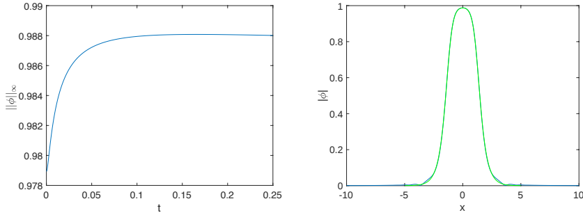
FIGURE 5. On the left the L^\infty norm of the solution of Fig. 4, on the right the solution at the final time in blue and a fitted ground state in green.
