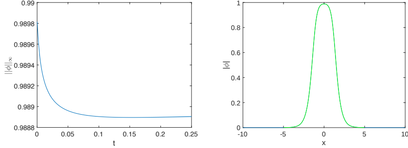
FIGURE 7. On the left the L^\infty norm of the solution of Fig. 4, on the right the solution at the final time in blue and a fitted ground state in green.
