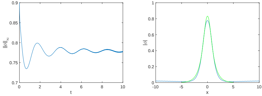
FIGURE 16. On the left the L^\infty norm of the solution of equation (1) for \alpha = 2 and the initial data \phi(x, 0) = 0.9 \exp(-x^2) , and the solution for t = 10 on the right in blue together with some fitted ground state in green.
