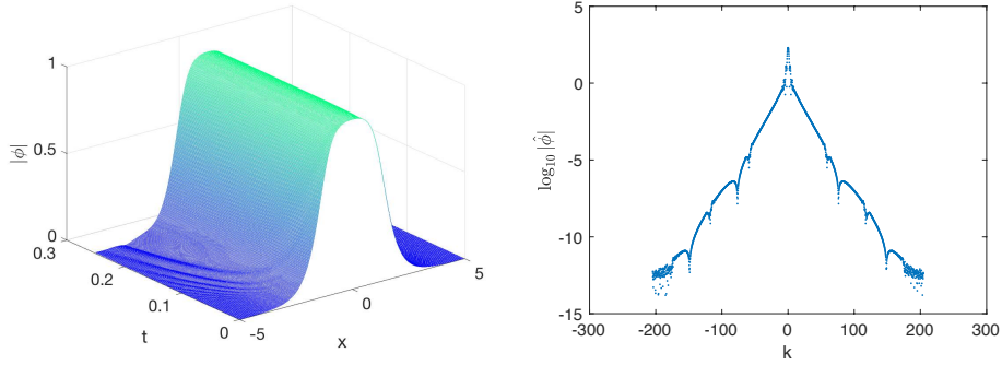
FIGURE 4. Solution to the equation (5) for the initial data \phi(x, 0) = 0.99\varphi(x, a = 9, b = 4.4) and \alpha = 1 on the left, and the Fourier coefficients of the solution at the final time on the right.
