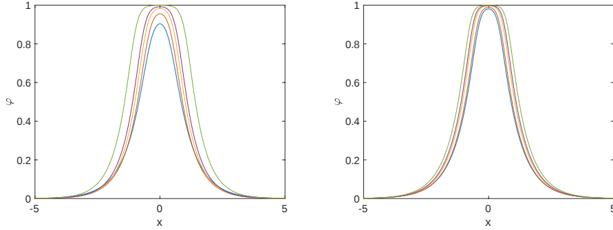
FIGURE 2. Ground state solution to equation (3) for a = 9 and \alpha = 2 on the left ( b = 2.0, 2.5, 2.8, 2.9 and 2.99 from bottom to top), and for \alpha = 3 on the right ( b = 2.0, 2.1, 2.2, 2.22 and 2.24 from bottom to top).
