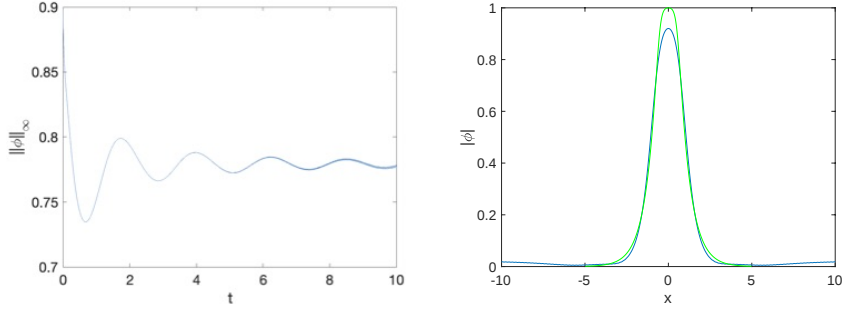
FIGURE 15. On the left the L^\infty norm of the solution of Fig. 14, on the right the solution at the final time in blue together with a fitted ground state in green.
