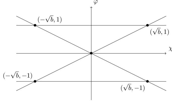
FIGURE 18. \Gamma_0 when a = (\alpha + 1)b
