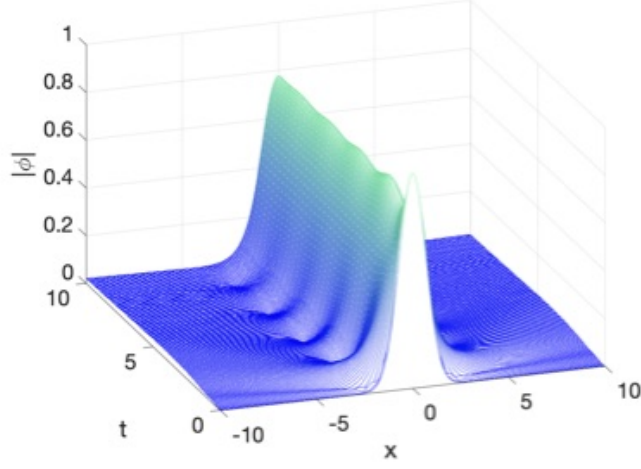
FIGURE 14. Solution to the equation (5) with a = 9 for the initial data \phi(x, 0) = 0.9 \exp(-x^2) .
