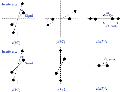
Figure 1. SAIC concept for BPSK signal and interference
