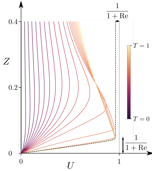
FIGURE 2 Single wave streaming and downward mean flow propagation. Snapshots of the mean flow vertical profile are shown obtained by direct numerical resolution of Eq. (32) using Re = 25 . The stationary solution given by Eq. (35) is shown in dashed.
