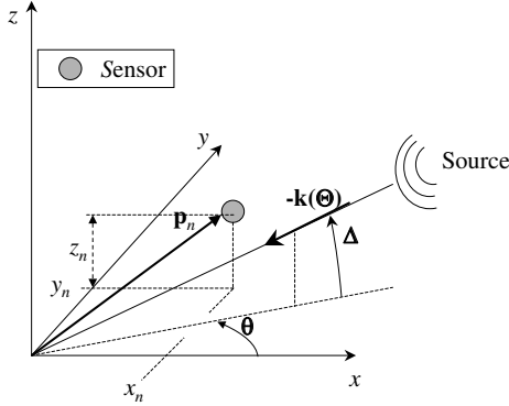
Figure 1: Source wave-vector \mathbf{k}(\Theta) of direction \Theta impinging the n -th sensor located at \mathbf{p}_n = [x_n \ y_n \ z_n]^T .
