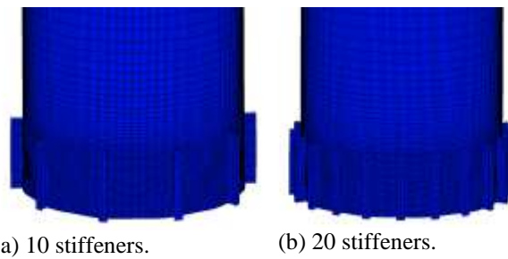
Figure 13. Shape mode for model 8.
