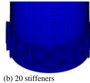
Figure 6. FEM model for the cylinders using the 1 st buckling mode (Model 7).
