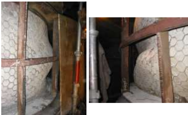
Figure 1. Typical deformation patterns at the riser bottom. Source: The authors.
