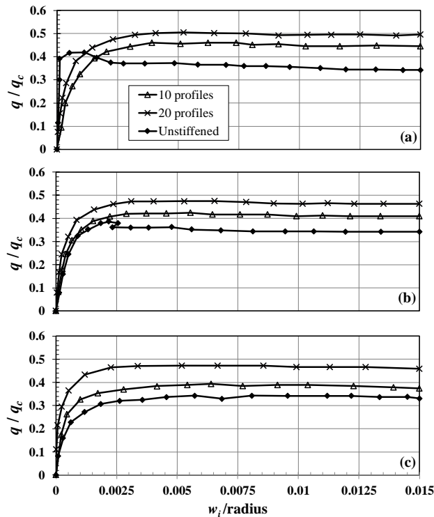
Figure 14. Ultimate buckling load for model 10: (a) Mode 1; (b) Mode 2; and (c) Mode 3.
