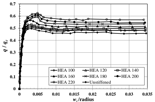
Figure 11. Effect of the HEA stiffeners on the ultimate buckling load.
