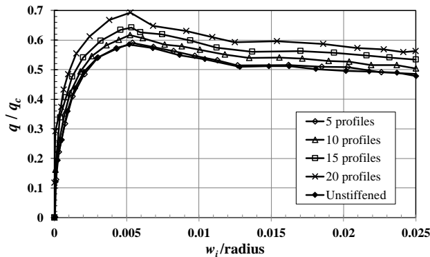
Figure 12. Influence of the number of profiles on the ultimate buckling load of Model 8.
