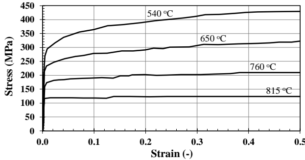
Figure 5. Elastoplastic behavior of a steel ASTM 240-304H under various temperatures.
