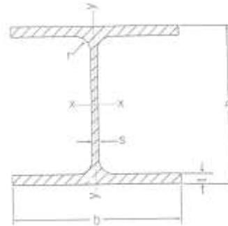
Figure 7. Profile HEA according to DIN 1025. (ASTM A - 6).
