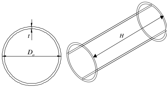
Figure 2. Geometry of the cylinders. Source: The authors.
