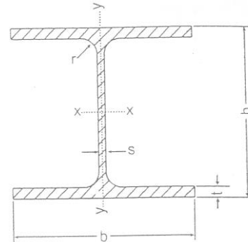
Figure 7. Profile HEA according to DIN 1025. (ASTM A - 6).
