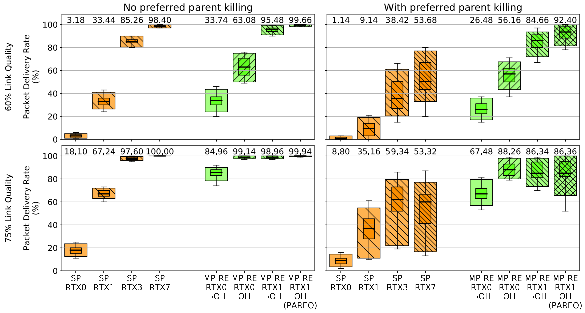
Fig. 4. Packet Delivery Rate (PDR). The four quadrants express the four combinations of the preferred parent killing (with and without) and the link quality (60% and 75%) parameters. In each plot, the orange boxes correspond to the default Single-path RPL routing algorithm, while the green to our Multi-path with RE routing algorithm. Furthermore, the outer (lighter) box corresponds to the 5%-95% percentiles, the inner (darker) to the 25%-75% percentiles, the middle line to the median and the whiskers represent the minimum and maximum. On top of each box, the mean value is presented. Finally, in the labels, OH and -OH stand for with and without the overhearing feature, and RTX_n expresses the number of re-transmissions performed.
