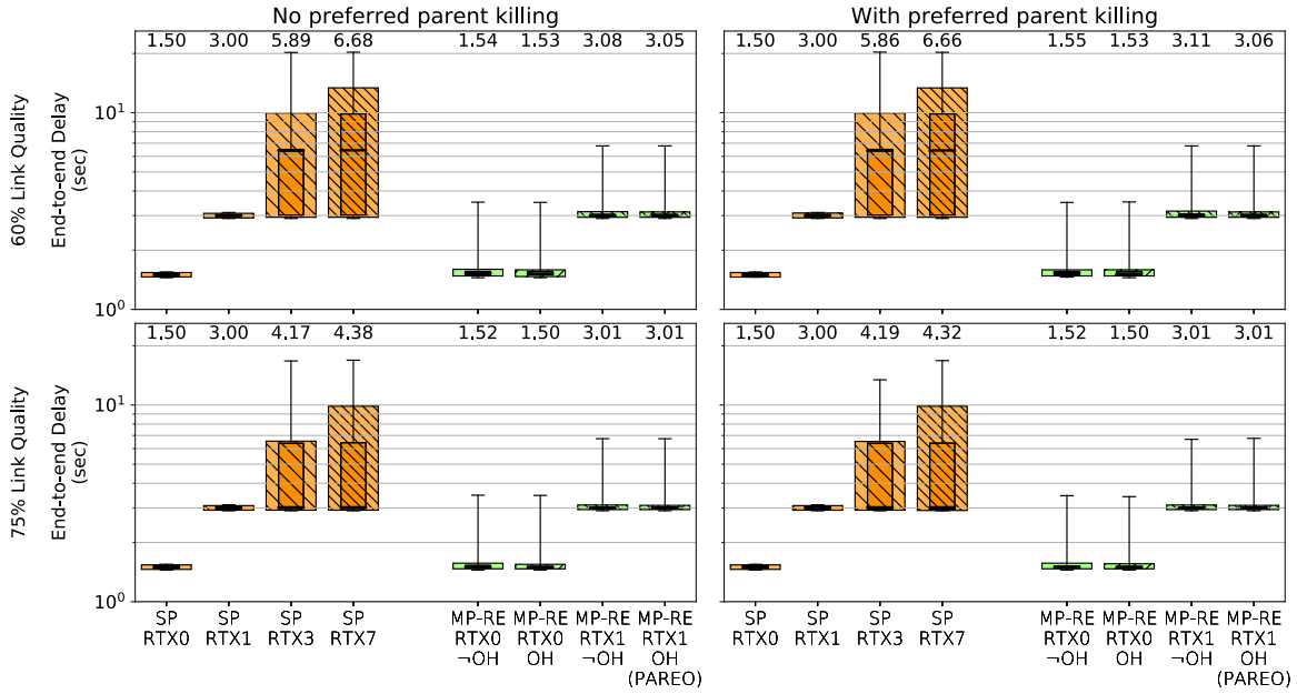
Fig. 5. Delay and Jitter (Percentiles of Delay). The four quadrants express the four combinations of the preferred parent killing (with and without) and the link quality (60% and 75%) parameters. In each plot, the orange boxes correspond to the default Single-path RPL routing algorithm, while the green to our Multi-path with RE routing algorithm. Furthermore, the outer (lighter) box corresponds to the 5%-95% percentiles, the inner (darker) to the 25%-75% percentiles, the middle line to the median and the whiskers represent the minimum and maximum. On top of each box, the mean value is presented. Finally, in the labels, OH and -OH stand for with and without the overhearing feature, and RTX n expresses the number of re-transmissions performed.
