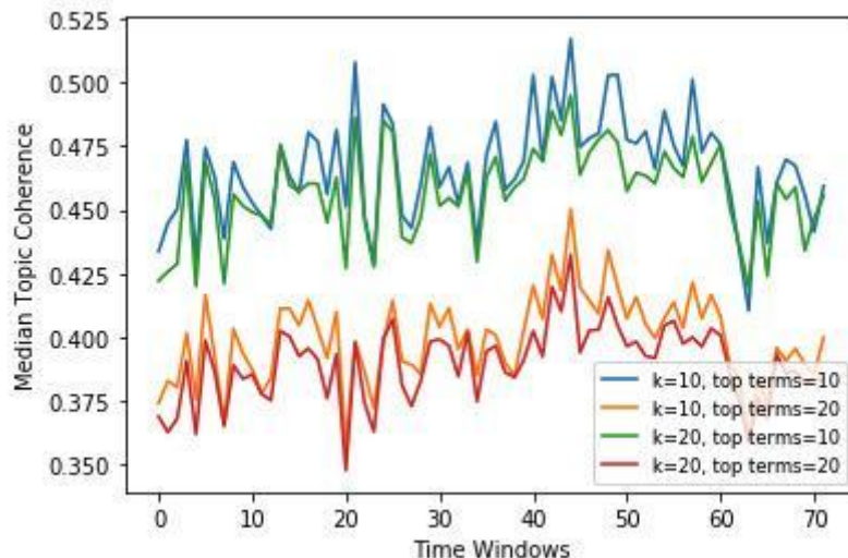
Figure 3. Median coherence scored calculated for 10 and 20 topics based on 10 and 20 top ranked topic descriptors for BJP in 1854-1925.
