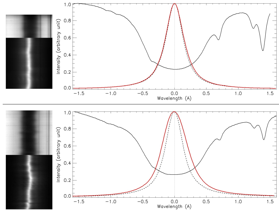
Figure 6. Calibration at F/60 of the two H\alpha filters ( 0.34 \text{ \AA} FWHM top, 0.46 \text{ \AA} FWHM bottom). Left: H\alpha observed line at disk center with or without the filter. Right: transmission functions; black line: observed line profile; dashed line: local typical transmission ( 0.32 \text{ \AA} FWHM); red line: global transmission averaged over the filter surface for pupil plane application.
