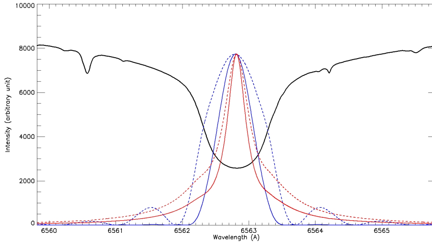
Figure 10. Spectral energy transmitted by old H\alpha Meudon Lyot prototypes (blue, 1985-2004 solid, 1965-1984 dashed) and the two DayStar Fabry Péro etalons (red, solid and dashed).
