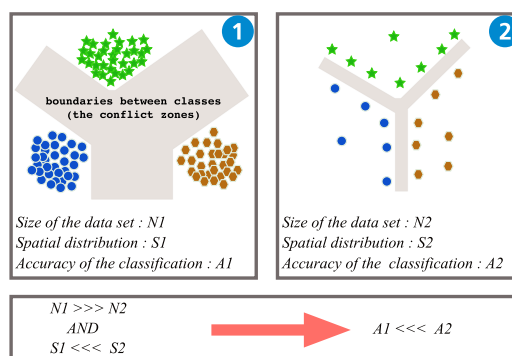
FIGURE 1. Basic illustration of an arbitrary 2D-representation of two different training data sets with two different spatial distributions. The data set #1 has more samples than the data set #2 but the accuracy of the classification is better for the data set #2.
