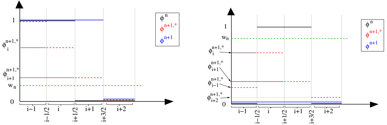
(a) Classical front propagation with the GRU step considering a first step based on a monotonicity preserving scheme. The initial front is located at interface i + 1/2 . For a first step of the algorithm based on a monotonicity preserving scheme, the GRU step consists in choosing on which interface i - 1/2, i + 1/2 or i + 3/2 the new front could be located at time t^{n+1} .
