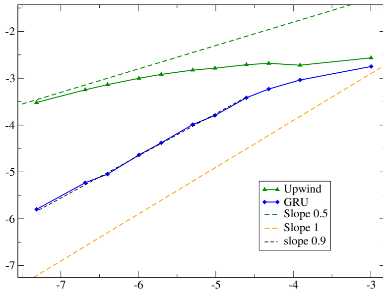
Figure 20: Convergence curves for the non-solid rotation of the non-convex Zalesak's shape on structured mesh. The green line represents the results for the sole Upwind scheme, whereas the blue line stands for the Upwind-GRU scheme.
