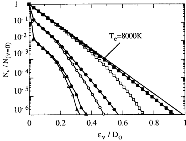
FIG. 3. Temporal relaxation of the vibrational level populations for T_e=8000 K with, at t=0 s, all the N_2 molecules populated in the ground state. The number density N_v is normalized by the number density on the ground state and \epsilon_v by the dissociation energy D_0 of N_2 . The time t is normalized by \tau_{eLee} calculated at T_e=8000 K. Closed symbols correspond to the harmonic oscillator approximation; open symbols correspond to the anharmonic oscillator approximation. Triangles, t=10^{-2}\tau_{eLee} ; circles, t=10^{-1}\tau_{eLee} ; squares, t=\tau_{eLee} . The solid line corresponds to the final Boltzmann distribution at T_e . This equilibrium is reached at t=7.2\tau_{eLee} in the harmonic case and at t=1363\tau_{eLee} in the anharmonic case.
