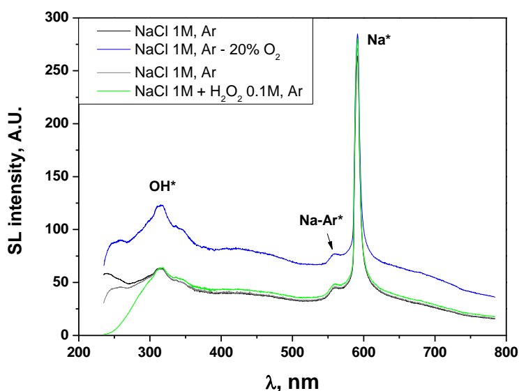
Fig. 8: SL spectra of a 1 M NaCl solution under Ar, Ar-20% O 2 and Ar after addition of 0.1M H 2 O 2 .
