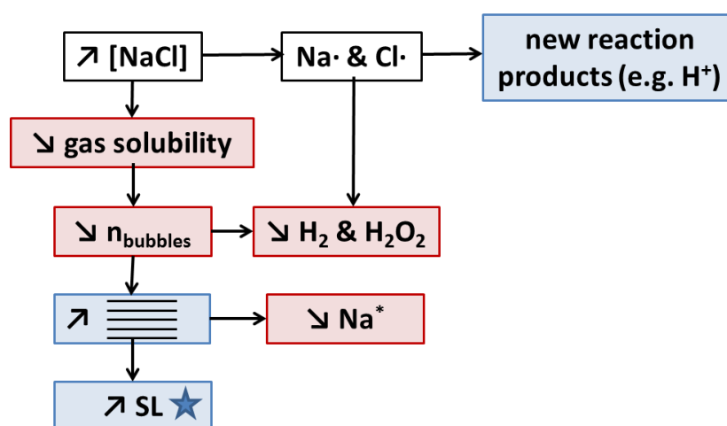
Fig. 10: Schematic representation of the different impacts of salt on sonochemistry and sonoluminescence.
