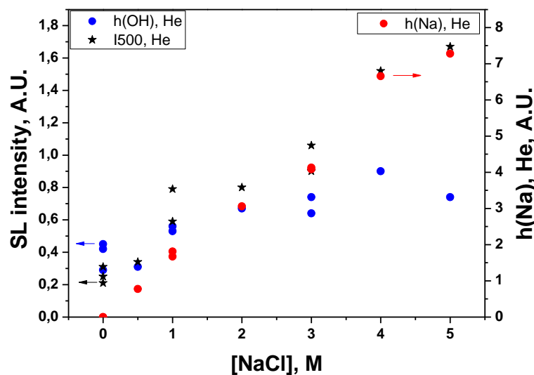
Fig. 5: Evolution with NaCl concentration of the SL continuum intensity, taken at 500 nm, of OH ( A^2\Sigma^+-X^2\Pi ) transition emission intensity and of Na^* line intensity, for Ar (a) and He (b).
