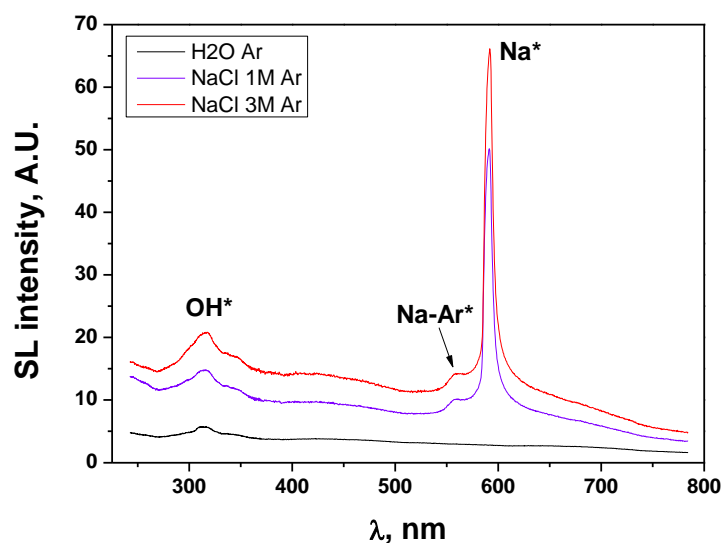
Fig. 4: Measured SL spectra under Ar flow, in water and in 1 M and 3 M NaCl aqueous solutions (362 kHz, 43 W, 10°C).
