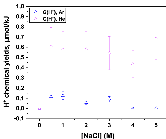
Fig. 2: Yields of H^+ formed during the sonolysis of NaCl solutions under Ar or He (362 kHz, 43 W, 13°C).
