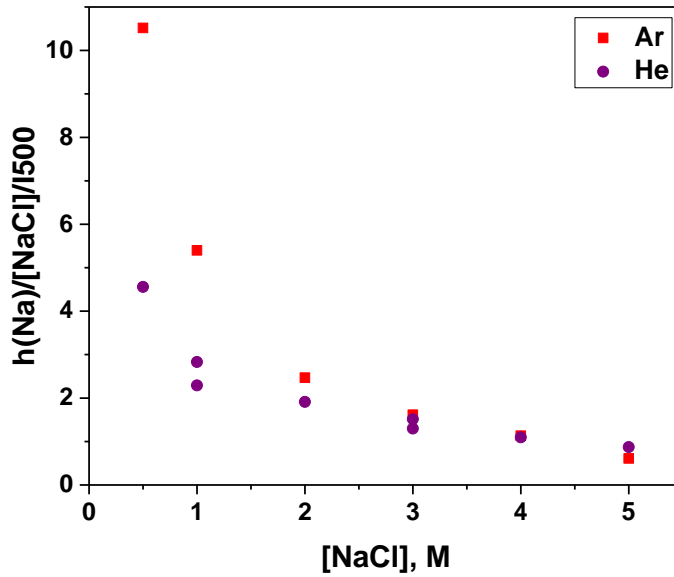
Fig. 9: Evolution with NaCl concentration of \text{Na}^* line intensity normalized by NaCl concentration, relative to the continuum intensity, taken at 500 nm, under He and Ar flows.
