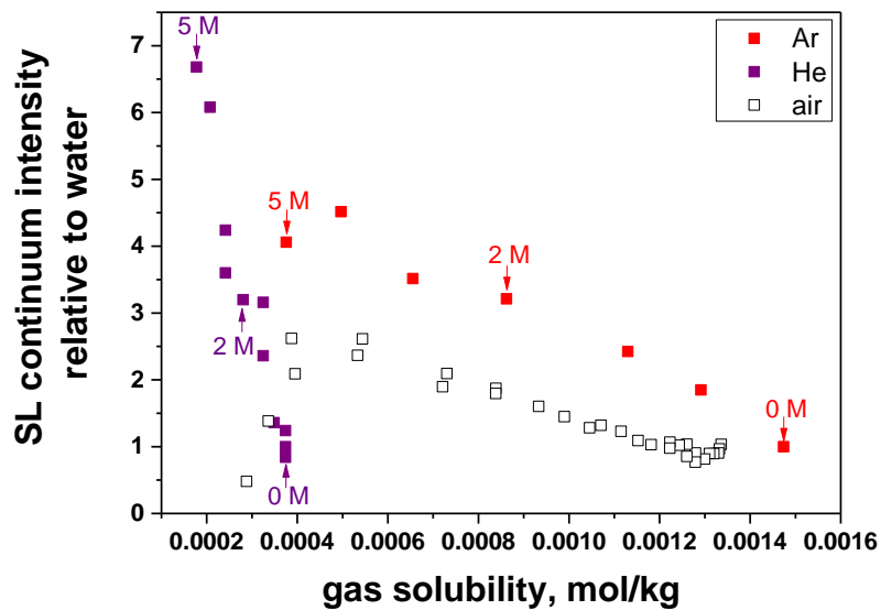
Fig. 6: Evolution of the SL continuum intensity (normalized to water) with the gas solubility for Ar, He and air (for air: literature values 11 ).
