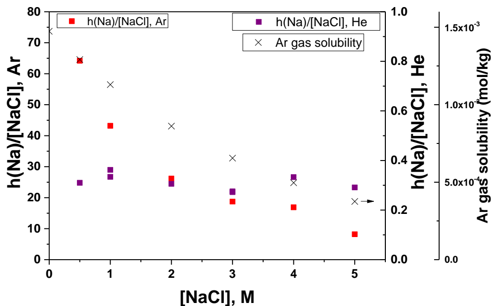
Fig. 7: Evolution with NaCl concentration of Na* line emission relative to NaCl concentration (A.U.), under He and Ar flows (values corrected to consider the same spectral acquisition time of 60 s), and of Ar solubility (He solubility is given in Fig. 5SI).
