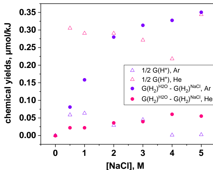
Fig. 3: Comparison of the yields of H + (G(H + )) formed during the sonolysis of NaCl solutions under Ar or He (362 kHz, 43 W, 13°C) with a decrease in H 2 yields between water and NaCl solutions (G(H 2 ) H 2 O -G(H 2 ) NaCl ).
