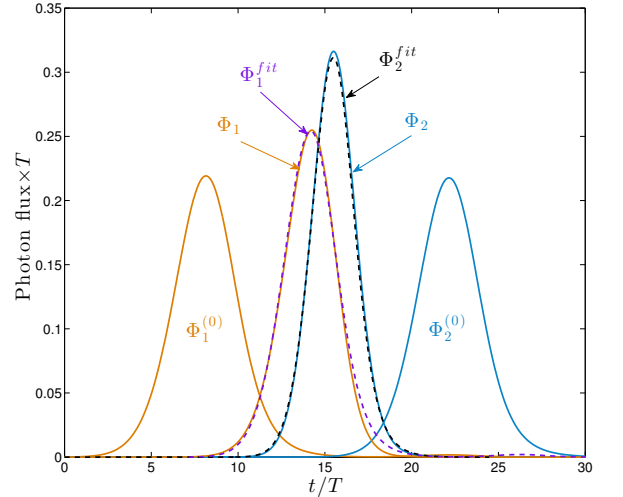
FIG. 9. Photon flux fit (dashed lines) of the partially overlapping photon fluxes ( \Phi_1 \equiv \Phi_{fg;gf,1} , \Phi_2 \equiv \Phi_{ff,1} in Fig. 8), using non overlapping flux shapes ( \Phi_1^{(0)} \equiv \Phi_{gf,1} , \Phi_2^{(0)} \equiv \Phi_{ff,1} in Fig. 7).
