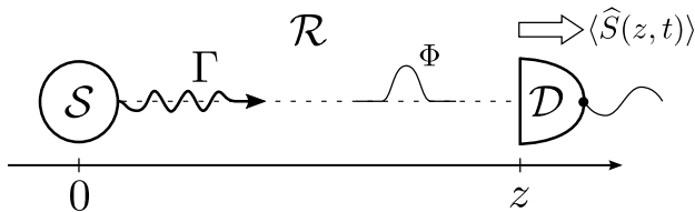
FIG. 2. Sketch of the photodetection: the source system \mathcal{S} emits a photon with decay rate \Gamma at position 0, towards a detector \mathcal{D} at a position z through the reservoir \mathcal{R} . The photon flux \Phi is measured using the data on the averaged quantum Poynting vector \langle \hat{S}(z, t) \rangle .
