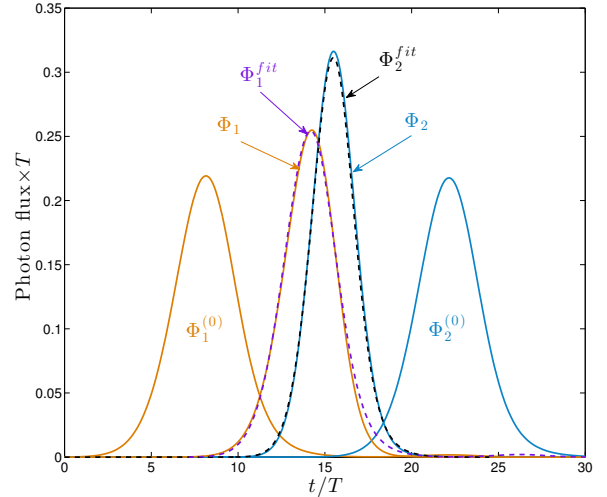
FIG. 9. Photon flux fit (dashed lines) of the partially overlapping photon fluxes ( \Phi_1 \equiv \Phi_{fg;gf,1} , \Phi_2 \equiv \Phi_{ff,1} in Fig. 8), using non overlapping flux shapes ( \Phi_1^{(0)} \equiv \Phi_{fg,1} , \Phi_2^{(0)} \equiv \Phi_{ff,1} in Fig. 7).
