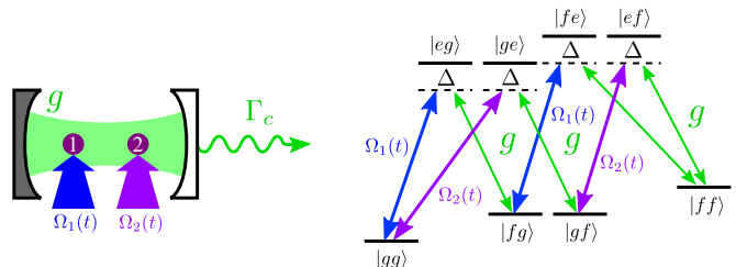
FIG. 5. 2-atom-cavity system. States |i\rangle \otimes |j\rangle \equiv |ij\rangle , i, j = g, e, f describe \Lambda -atoms 1 and 2. Rabi frequencies \Omega_k , k = 1, 2 drive the transitions |g\rangle \rightarrow |e\rangle .
