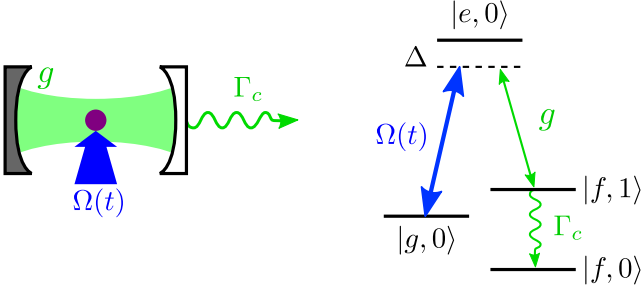
FIG. 3. Atom-field interaction in the cavity: (left panel) a single \Lambda -atom is driven by an external classical laser field of Rabi frequency \Omega , and a quantized cavity field with coupling strength g . (Right panel) The fields are in two-photon resonance, the one-photon detuning is \Delta . Initially the atom is in the ground state |g\rangle . In the course of the excitation process, one photon is taken from the laser field and transferred to the cavity, which eventually leaks out of the cavity through a semi-transparent mirror characterized by the decay rate \Gamma_c .
