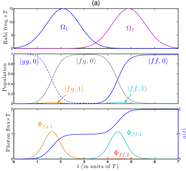
FIG. 7. (Upper panel) Rabi frequencies (in units of T ) of delay 2\tau = 2.8T . (Middle panel) Populations in the dressed basis for (\Omega_0, \Delta, g, \Gamma_c) \times T = (15, 100, 40, 40) . (Lower panel) Outgoing photon flux \Phi = \Phi_{fg,1} + \Phi_{ff,1} + \Phi_{ff,2} (in units of T ) and outgoing photon number (dark blue).
