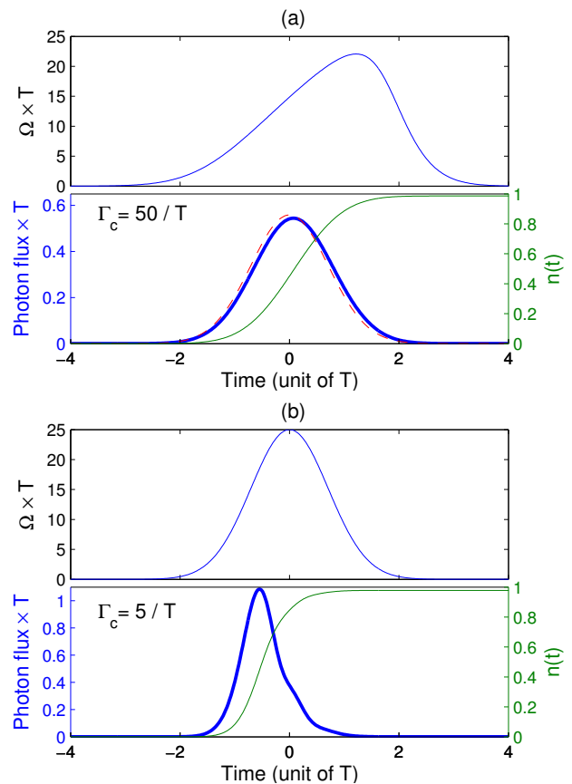
FIG. 4. (a) Rabi frequency \Omega(t)T (32) with (g, \Gamma_c, \Delta) \times T = (25, 50, 100) , \eta = 0.99 , determined from the desired Gaussian shape flux \Phi(t) (33) [desired (dashed line) and numerical from the original model (26) (thick line)] of the single photon through the semi-transparent mirror (in units of T ); number of outgoing photons n = \int_{-\infty}^t dt' \Phi(t') = \Gamma_c \int_{-\infty}^t dt' |c_{f,1}(t')|^2 during the process (thin line). (b) Same as above but for \Gamma_c = 5/T and a chosen Gaussian Rabi frequency \Omega(t) = 25 \exp[-t^2/T^2]/T .
