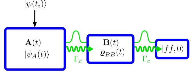
FIG. 6. Dynamical map of a two-atom system driven by two laser fields and trapped in a cavity. The dynamics splits into 3 blocks [from left to right, \mathbf{A} , \mathbf{B} , and \{0\} , see Eq. (34)] connected by the cavity decay rate \Gamma_c = 2\pi\kappa^2 .
