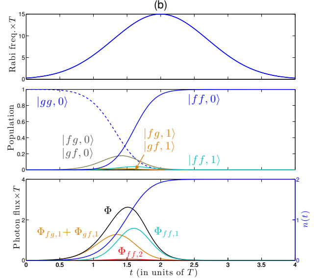
FIG. 8. Same as Fig. 7 but for \Omega_1(t) = \Omega_2(t) .
