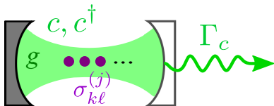
FIG. 1. Representation of the CQED system: N atoms are coupled to a single cavity mode of annihilation-creation operators c, c^\dagger , with the atom-cavity coupling g . Each operator \sigma_{k\ell}^{(j)} corresponds to the |k\rangle \leftrightarrow |\ell\rangle , k, \ell = g, e, f transition of the j -th atom, and photons leak through the right semitransparent mirror with decay rate \Gamma_c .
