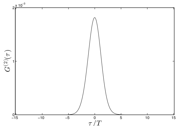
FIG. 10. Unnormalized two-time second order correlation function G^{(2)}(t_{\text{peak}}, \tau) \equiv G^{(2)}(\tau) , with respect to the reference time t_{\text{peak}} corresponding to the maximum of \Phi(t) .
