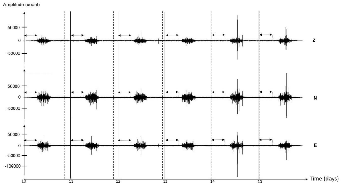
Figure 6. Synthetic seismograms from January 10 to January 15, 2019, compiled by a group of students. Vertical black lines: start of a new terrestrial day. Vertical black dashed lines: start of a new martian sol. Double arrows with black dashed vertical segments: marker of the lag between midnight (UTC) and the start of the middle daily event on January 10, 2019. From January 11 to January 15, students observed that the lag increased day after day. E: East component. N: North component. Z: vertical component.
