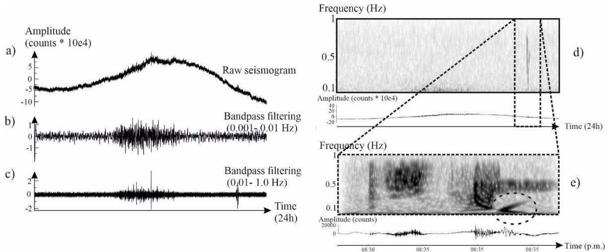
Figure 3. Synthetic marsquake on January 12, 2019 (vertical component). (a) Raw seismogram. (b) Raw seismogram filtered with bandpass filtering from 0.001 Hz to 0.01 Hz. (c) Raw seismogram filtered with bandpass filtering from 0.01 Hz to 1.0 Hz. (d) Raw seismogram and corresponding spectrogram. (e) An enlargement of the black dashed rectangle in (d). Black dashed ellipse: supposed frequency signature of Rayleigh waves.
