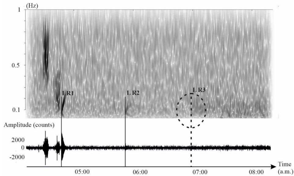
616 Figure 7. Study of the unknown event detected by students on July 15, 2019. Raw seismogram 617 filtered with bandpass values from 0.1 Hz to 1.0 Hz and the corresponding spectrogram. 618 Vertical black lines: pick of Rayleigh waves clearly identified in the spectrogram. Vertical black 619 dashed line: pick of LR3 hypothesized by students.
