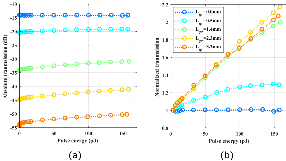
FIG. 5. (a) Absolute transmission as a function of the coupled pulse energy ( I_{\text{ampli}} = 160 mA, \tau_{\text{FWHM}} = 0.2 ps, 20 MHz, 1547 nm) for \text{Si}_3\text{N}_4 waveguides covered by different graphene lengths. (b) Related normalized transmission for the same series of waveguides, where each transmission curve is normalized by the corresponding transmission at low pulse energy ( E_{\text{pulse}} = 3 pJ).
