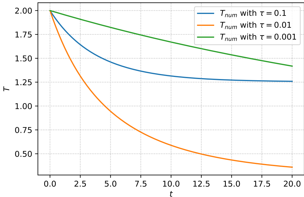
Haff's cooling law for e = 0.9 with different aus .
