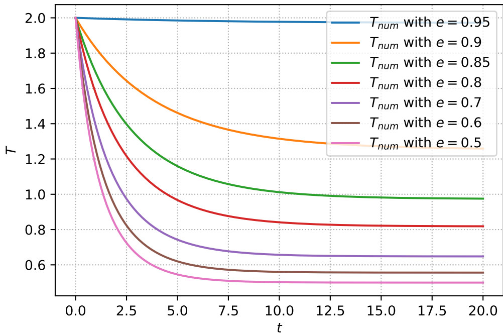
Haff's cooling law with a maxwellian as initial.
