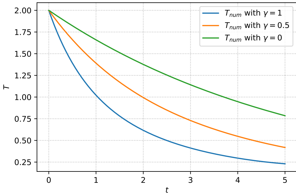
Haff's cooling law for e = 0.5 (without heat bath).
