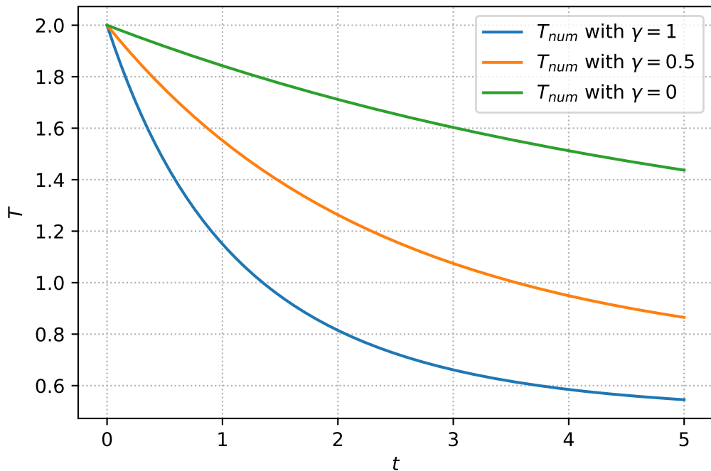
Haff's cooling law for e = 0.5 (with heat bath).
