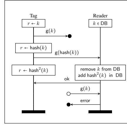
Fig. 4. Linkability attack for OSK protocol
