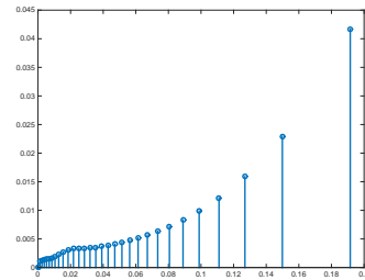
Fig. 4. Release instants and release interval by event-triggering
