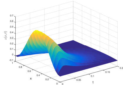
Fig. 3. State of the closed-loop system with the event-triggered control law (2.3) distributed over all domain
