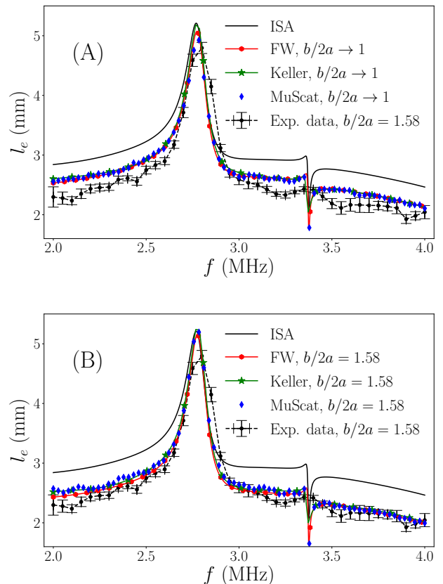
FIG. 4. (Color online) Scattering mean free path of a slab with concentration \phi = 14\% , and b/2a \rightarrow 1 (A) or b/2a = 1.58 (B) - comparison between experimental results, MuScat simulations and homogenization calculations. Frequency range corresponds to ka \in [3.35 - 6.7] .
