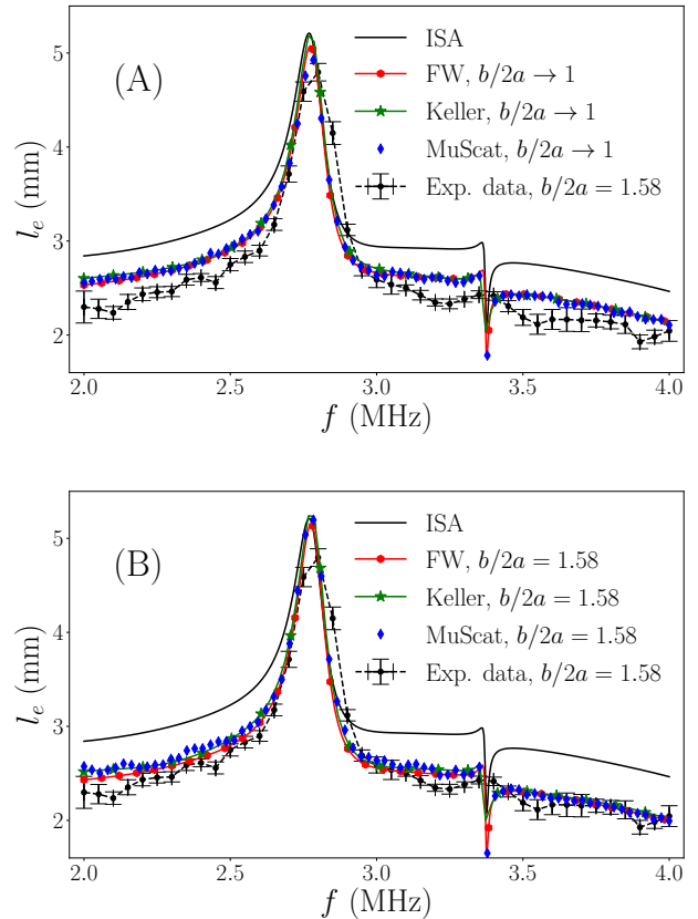
FIG. 4. (Color online) Scattering mean free path of a slab with concentration \phi = 14\% , and b/2a \rightarrow 1 (A) or b/2a = 1.58 (B) - comparison between experimental results, MuScat simulations and homogenization calculations. Frequency range corresponds to ka \in [3.35 - 6.7] .
