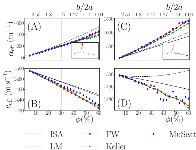
FIG. 6. (Color online) Effective attenuation and phase velocity as a function of the concentration, for frequency f = 2.77 MHz, ka = 4.64 ((A), (B)), which corresponds to a resonance frequency, and f = 4 MHz, ka = 6.7 ((C), (D)). The dots on the subplots show the relative position on the spectrum of Fig. 3 and Fig. 4. The vertical dotted line corresponds to the concentration chosen to calculate effective parameters of Fig. 5.
