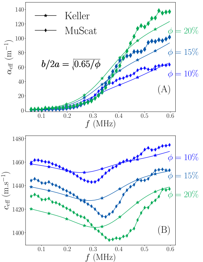
FIG. 9. (Color online) Effective attenuation and phase velocity as a function of the frequency for b/2a = \sqrt{0.65/\phi} and various concentrations. Frequency range corresponds to ka \in [0.1 - 1.0] .
