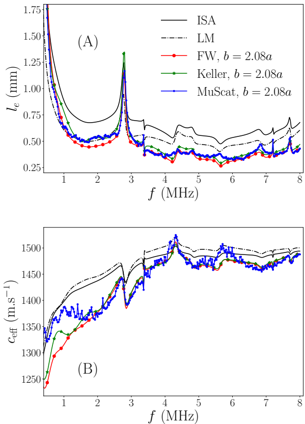
FIG. 7. (Color online) Scattering mean free path (A) and effective phase velocity (B) calculated with MuScat (diamonds markers), Keller, FW, ISA and LM models for concentration \phi = 60\% . Frequency range corresponds to ka \in [1.0 - 13.4] .
