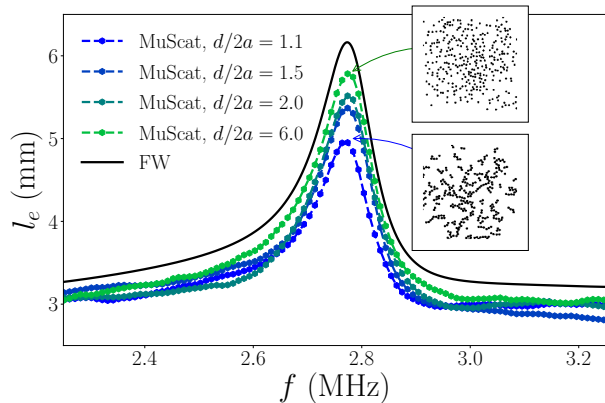
FIG. 10. (Color online) Scattering mean free path for heterogeneous media with different cluster types, with a concentration of \phi = 10\% . Frequency range corresponds to ka \in [3.77 - 5.44] .
