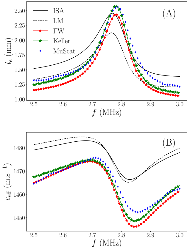
FIG. 5. (Color online) Effective attenuation (A) and effective phase velocity (B) for a concentration of \phi = 30\% , calculated with MuScat (diamond markers) and different statistic models : Linton and Martin (LM), Fikioris and Waterman (FW), ISA and Keller. Frequency range corresponds to ka \in [4.18 - 5.02] .
