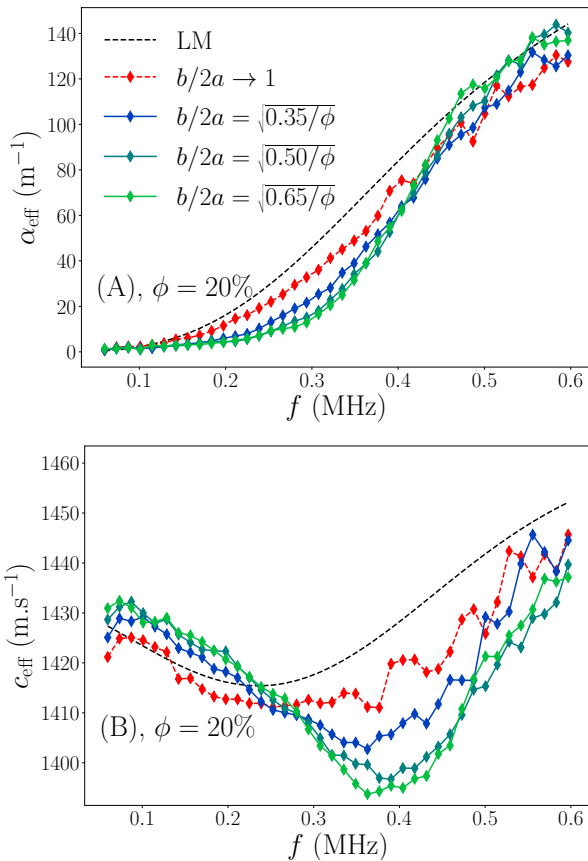
FIG. 8. (Color online) Effective attenuation and phase velocity as a function of the frequency for a concentration of \phi = 20\% and various values of b . Frequency range corresponds to ka \in [0.1 - 1.0] .
