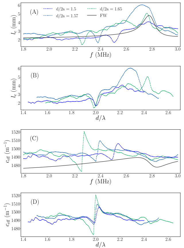
FIG. 11. (Color online) Effective parameters l_e and c_{eff} of slabs with crystal-like geometrical properties (crystal with defects), such as presented on figure 2, plotted as a function of frequency f (A), (C) and a function of d/\lambda (B), (D). Frequency range corresponds to ka \in [3.0 - 5.0] .
