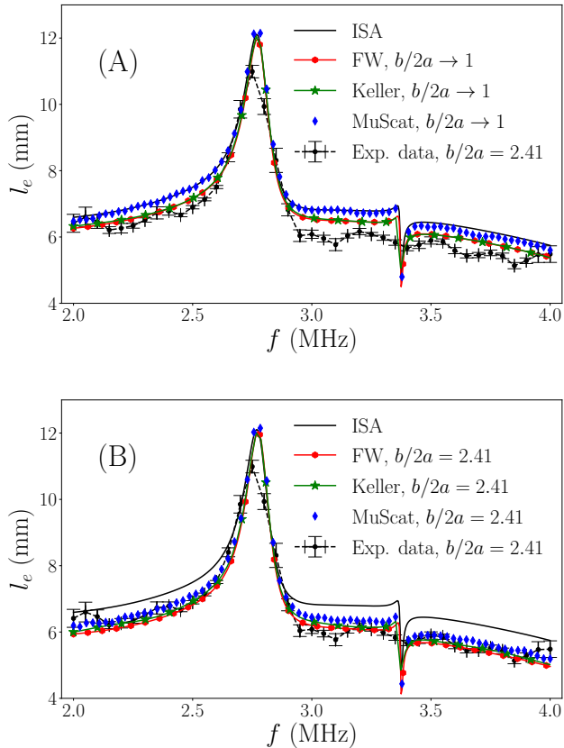
FIG. 3. (Color online) Scattering mean free path of a slab with density \phi = 6\% , and b/2a \rightarrow 1 (A) or b/2a = 2.41 (B) - comparison between experimental results, MuScat simulations and homogenization calculations. Frequency range corresponds to ka \in [3.35 - 6.7] .
