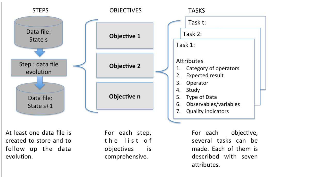
Figure 3: Generic description of the DC_TEL framework, with its steps, objectives, tasks and the attributes for the tasks.
