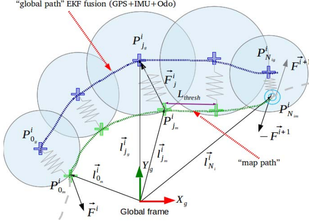
Fig. 5. Each map path point P_{jp}^i is attracted to its corresponding global path point P_{jg}^i with a force \vec{F}_j^i proportional to the inverse of the covariance of the error cov_j^i and the relative position between them \vec{l}_j^i . Note that in the connection point P_{Nm}^i the force between the connected sub-maps have same value but contrary direction by the principle of action and reaction
