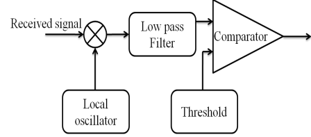
Fig. 3. Coherent ASK receiver.
