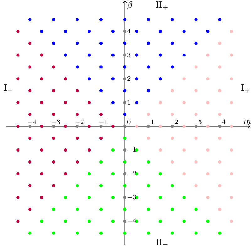
Figure 2: Solutions for the doubly degenerate case: Region I - : the decaying Laguerre and the exploding Laguerre solutions. Region I + : any of the three solutions. Region II + : the decaying Laguerre and the exploding logarithmic solutions. Region II - : the exploding Laguerre and the decaying logarithmic solutions.
