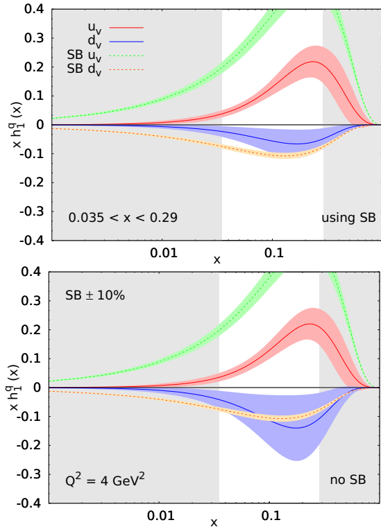
Figure 1: Transversity functions for u_v (red) and d_v (blue) flavours from a global fit to SIDIS and e^+e^- data at Q^2 = 4 \text{ GeV}^2 . Upper panel: results with automatic fulfillment of the Soffer Bound ( |N_{u_v(d_v)}^T| \leq 1 ). Lower panel: results with no constraint on N_{u_v(d_v)}^T . Error bands on the fitted functions are at 2\sigma level. The corresponding Soffer bound, computed with CTEQ66 [40] PDFs and DSSV [39] helicity distributions, is also shown for u_v (green) and d_v (orange), together with a \pm 10\% variation. The white area represents the region of the bulk of the data; outside it no data are included in the fit.
