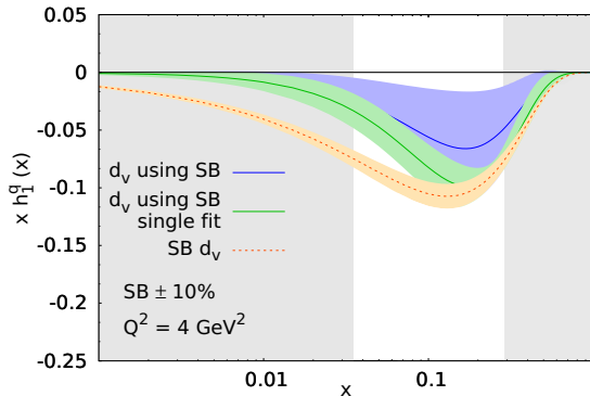
Figure 3: Transversity functions for d_v flavour from a global fit to SIDIS and e^+e^- data at Q^2 = 4 \text{ GeV}^2 . Blue band corresponds to usage of priors from Fig. 1, while green band corresponds to priors generated from constrained fit |N_{d_v}^T| \leq 1 directly. Error bands on the fitted functions are at 2\sigma . The corresponding Soffer bound, computed with CTEQ66 [40] PDFs and DSSV [39] helicity distributions, is also shown, together with a \pm 10\% variation. The white area represents the region of the bulk of the data; outside it no datapoints are present in the fit.
