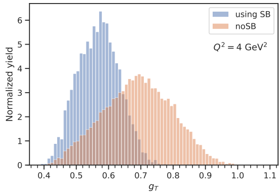
Figure 5: Distributions of the isovector tensor charge, g_T , at Q^2 = 4 \text{ GeV}^2 . The calculation is performed using the extracted transversity distributions of Fig. 1, integrated over the full range 0 \leq x \leq 1 . Labels “using SB” and “no SB” have the same meaning as in Fig. 1.
