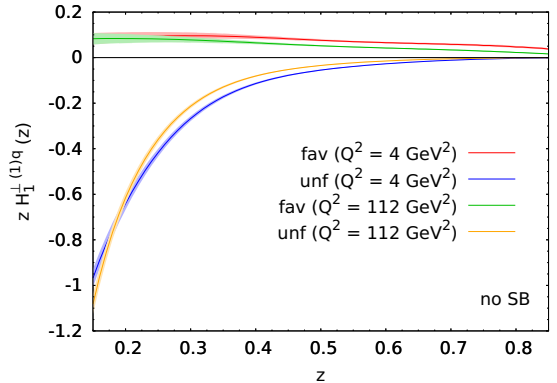
Figure 2: First moments of the favoured and unfavoured Collins fragmentation functions from a global fit to SIDIS and e^+e^- data for the “no SB” case. Curves at Q^2 = 4 \text{ GeV}^2 (red and blue) and Q^2 = 112 \text{ GeV}^2 (green and orange) are shown. Error bands on the fitted functions are at 2\sigma level. Notice that the results for the “using SB” case are practically the same.
