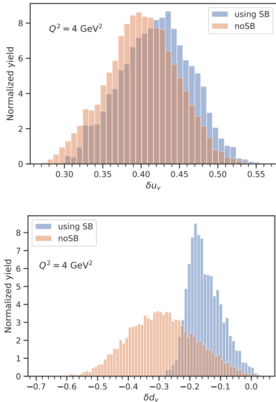
Figure 4: Distributions of the tensor charges for u_v (upper panel) and d_v (lower panel) at Q^2 = 4 \text{ GeV}^2 . The tensor charges are calculated using the extracted transversity distributions of Fig. 1, integrated over the full range 0 \leq x \leq 1 . Labels “using SB” and “no SB” have the same meaning as in Fig. 1.
