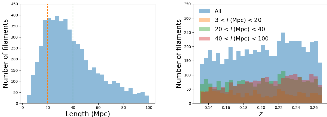
Fig. 3. Selection of the SDSS-DR12 LOWZCMASS DisPerSE filaments used. Left : three-dimensional length distribution. The orange dotted line shows the limit between the short and regular filaments, and the green dotted line shows the limit between the regular and long filaments. Right : redshift distribution of all filaments, overlaid with the redshift distributions of the filaments for the three bins of lengths.
