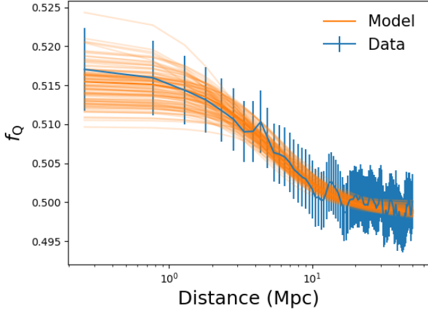
Fig. 10. In blue, the quiescent fraction profile f_Q , averaged around the 5559 selected filaments. In orange, the \beta -model (Eq. (5)) from different realisations of the MCMC.
