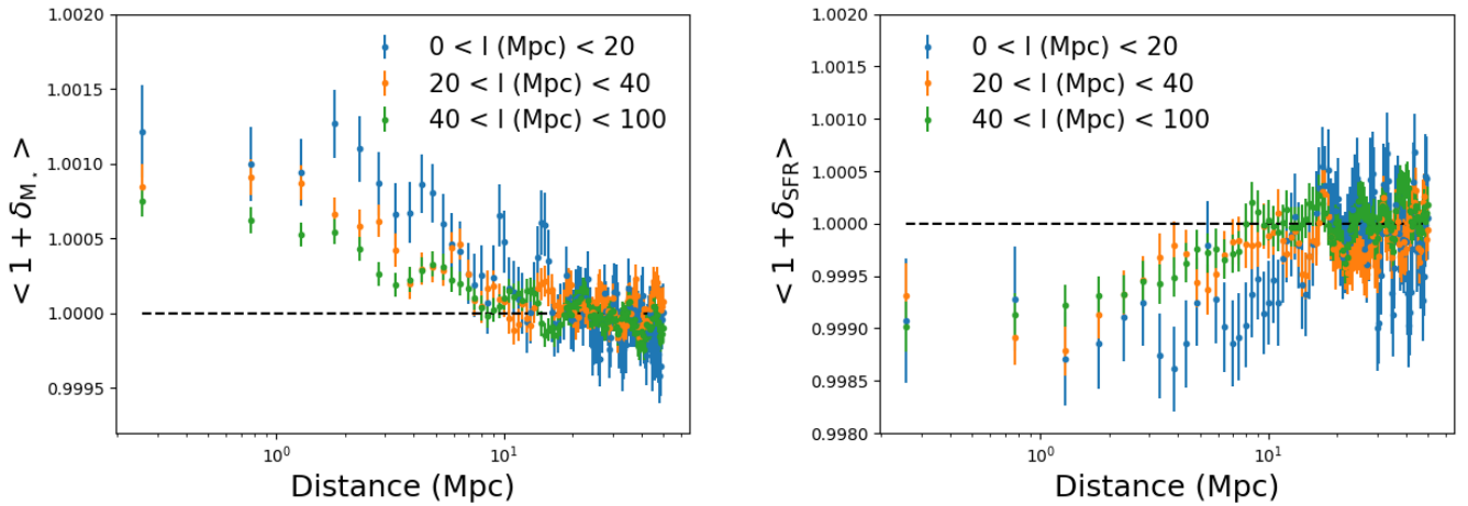
Fig. 7. Radial stacked profiles of excess of M_* and SFR: \langle 1 + \delta_{\text{SFR}} \rangle and \langle 1 + \delta_{M_*} \rangle for the short, regular, and long filaments.
