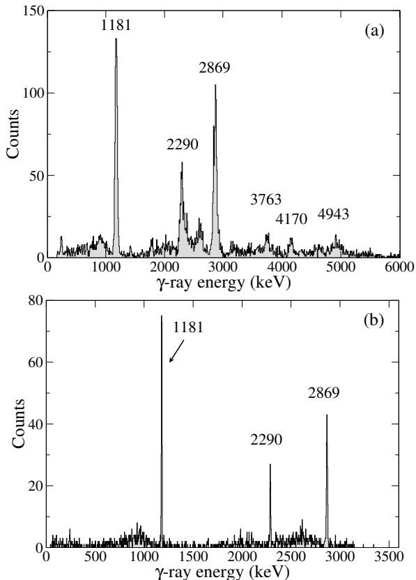
FIG. 4: \gamma -ray spectra obtained by slice of the [E^*(^{210}\text{Po}), E_\gamma] matrix close to the E^* = E_\gamma line as defined on Fig. 3, in order to isolate the direct gamma de-excitations towards the ^{210}\text{Po} ground state. (a) LaBr 3 data, (b) Ge data.
