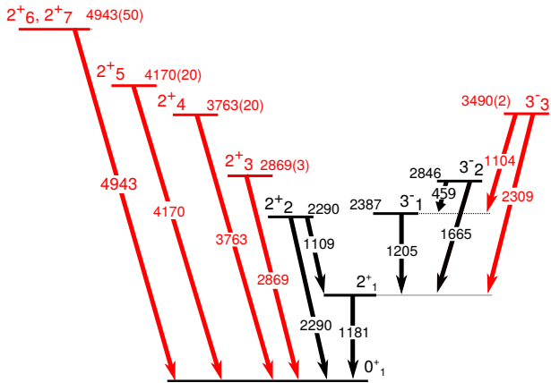
FIG. 7: (Color online) Partial level scheme of ^{210}\text{Po} exhibiting all the known 2^+ and 3^- excited states. Levels and \gamma rays identified in this work are displayed in color. All arrow widths are identical and do not represent the relative \gamma intensities.
