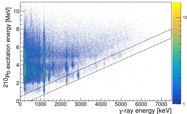
FIG. 3: (Color online) Two-dimensional plot of the [E^*(^{210}\text{Po}), E_\gamma] matrix, i.e. associated with a ^{10}\text{Be} identification in the Si telescopes (see text for details). The gamma rays have been detected in the LaBr 3 scintillators. The dashed lines are the contour limit of \pm 500 keV around the E^* = E_\gamma line which is used to obtain the projected gamma-ray spectrum shown in Fig. 4(a).
