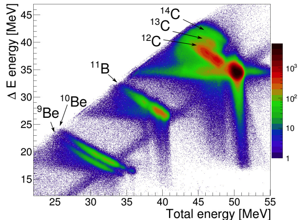
FIG. 2: (Color online) \Delta E - E spectrum for ejectiles measured by one pair of the \Delta E - E Si telescopes at E_{\text{beam}} = 63.7 MeV. Beam-like identified reaction products are labeled.
