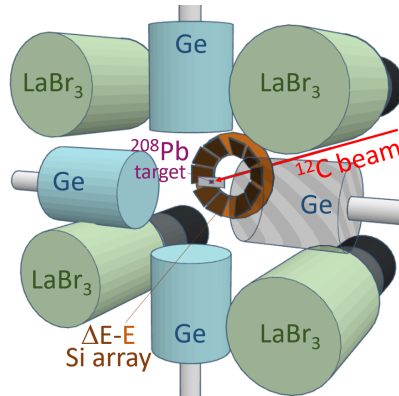
FIG. 1: (Color online) Schemactic view of the experimental setup used in this work.
