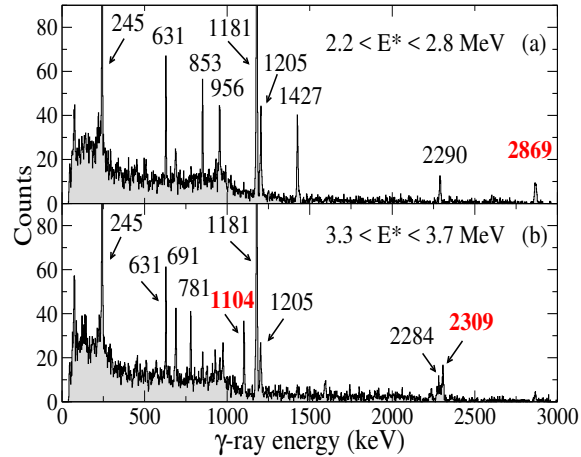
FIG. 6: (Color online) Gamma ray spectra obtained by slices of the [E^*(^{210}\text{Po}), E_\gamma] matrix, (a) E^* \in [2.2, 2.8] MeV, (b) E^* \in [3.3, 3.7] MeV. For clarity reason, the spectra have been vertically expanded, the peaks at 1181 keV ( 2_1^+ \rightarrow 0^+ ) and 245 keV ( 4_1^+ \rightarrow 2_1^+ ) are therefore cut. The new transitions observed in this work are labeled in bold.
