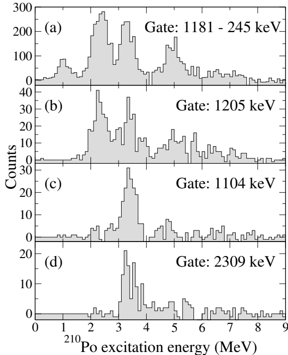
FIG. 5: ^{210}\text{Po} excitation energy distribution spectra obtained by slices of the [E^*(^{210}\text{Po}), E_\gamma] matrix: (a) LaBr 3 gate on the 2_1^+ \rightarrow 0^+ 1181-keV transition with subtraction of the feeding from the 4_1^+ \rightarrow 2_1^+ 245-keV transition, (b) Ge gate on the 3_1^- \rightarrow 2_1^+ 1205-keV transition, (c) Ge gate on the 1104-keV transition, (d) Ge gate on the 2309-keV transition.
