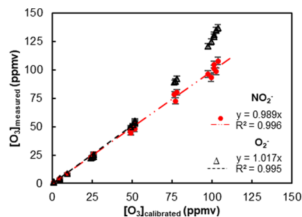
Figure 3. Comparison between the calibrated ozone concentrations with those measured by NO 2 - precursor ion (red ●) and O 2 - precursor ion (Δ).
