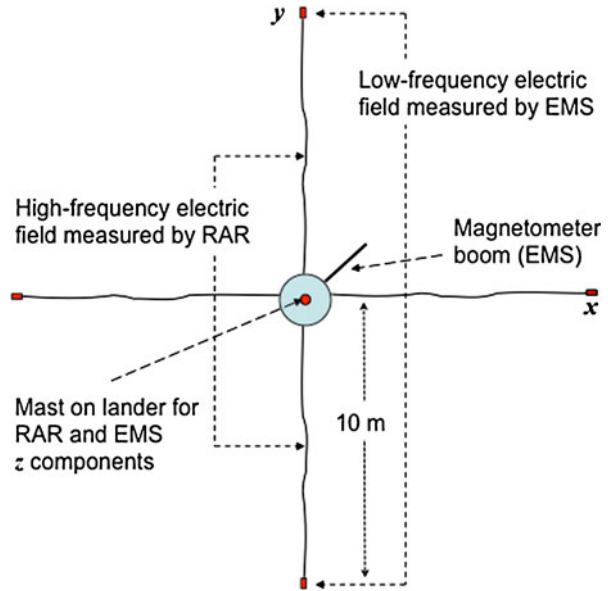
Fig. 16 The radio astronomy receiver (RAR) and electromagnetic sounding (EMS) experiment utilize the same antennas to measure all three components of the high- and low-frequency electric fields, respectively. RAR measures differences in voltage of the separate antennas, whereas EMS measures differences in voltage between the antenna end points
